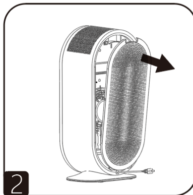
2 Use your hand to remove the rear case from the buckle.
